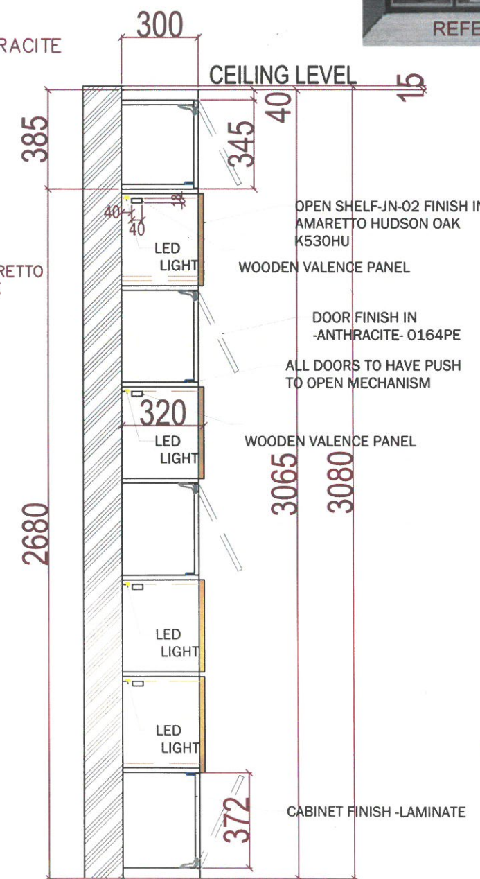
SECTION
