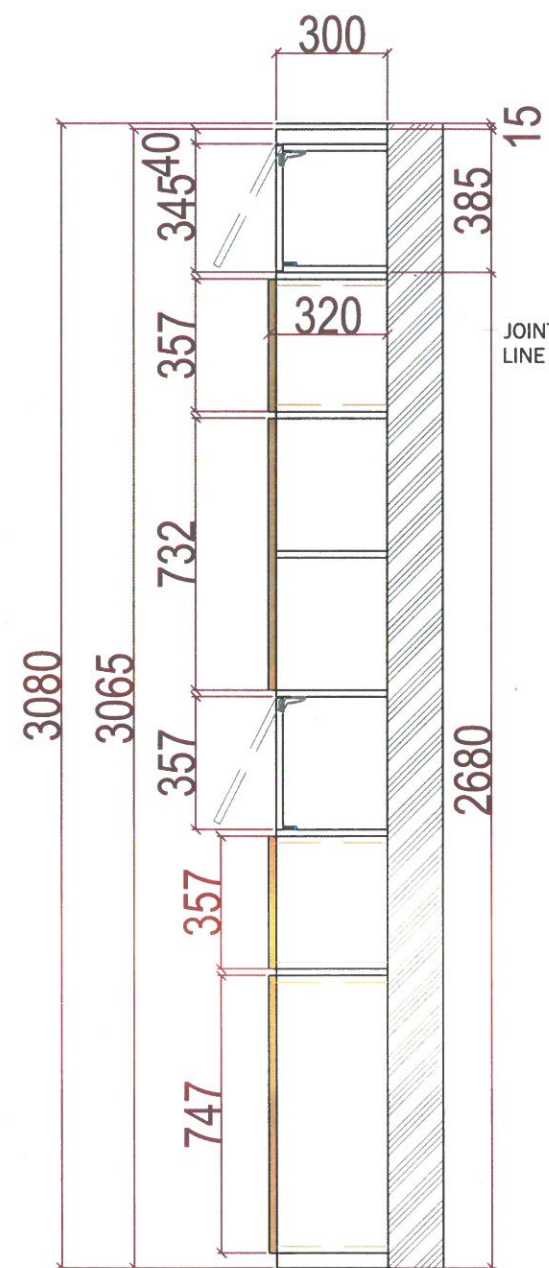
SECTION
